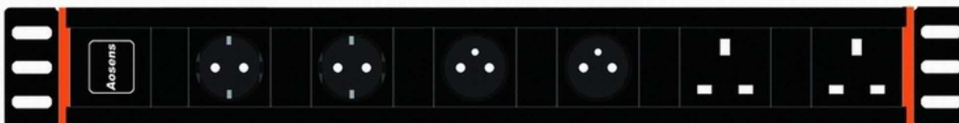
型号 Model: AS-1.5UB-G2F2E2 尺寸 Size: 430*66.6*44.4mm 额定电流 16-32A, 2位德标, 2位英标, 2位法标输出孔 16-32Amp rated current/2 German outlets outlets/2 France outlets/2 U.K. outlets outlets
