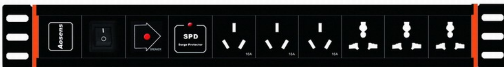
型号 Model: AS-1.5UB-M3J3KGF 尺寸 Size: 430*66.6*44.4mm 额定电流 16A, 3位10A万用孔, 3位16A国标孔, 总控开关(带指示灯), 过载保护, SPD防雷(浪涌)保护功能(带指示) 16Amp rated current/3 10-amp international outlets/3 16-amp Chinese outlets/ One 16-amp general control switch (indicator)/ One 16-amp overload protector/ One SPD LED
