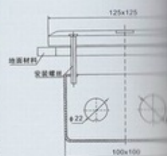
不锈钢屏蔽盖 Stainless steel shielding cover
