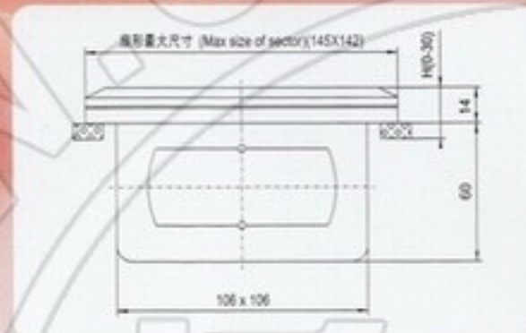
外形及安装尺寸 / Overall and installation size
