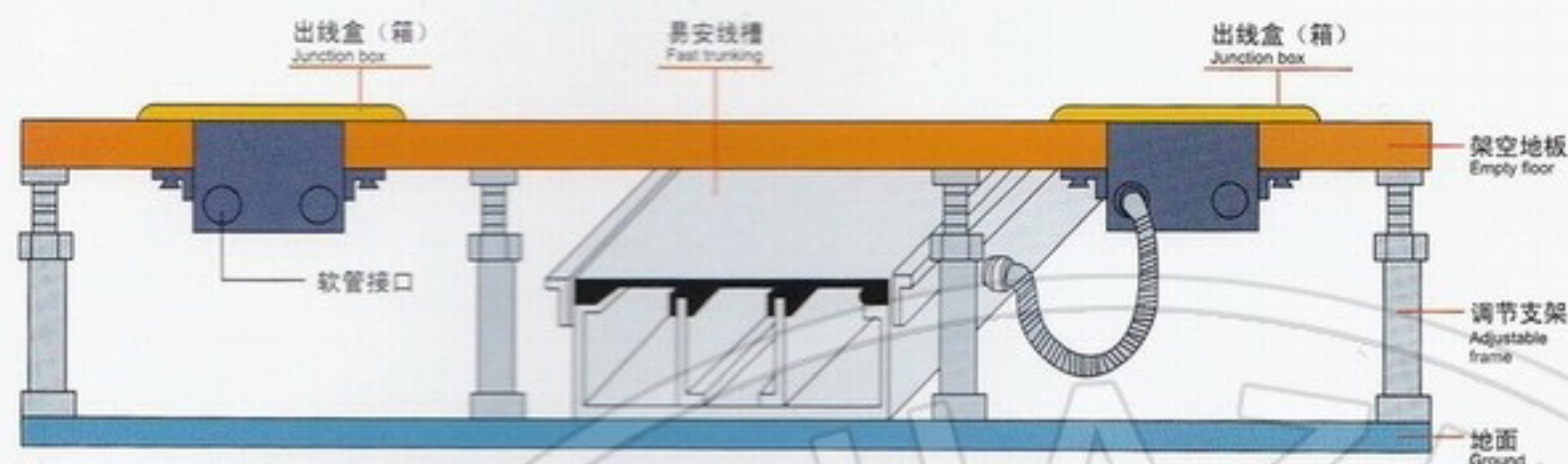
易安线槽与地毯面使用图例 The photo of fast trunking used in carpet
