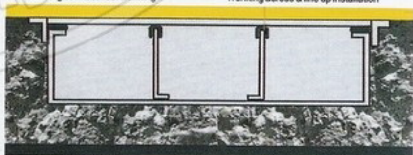
易安地面线槽剖面图 The cutaway view of fast floor trunking
