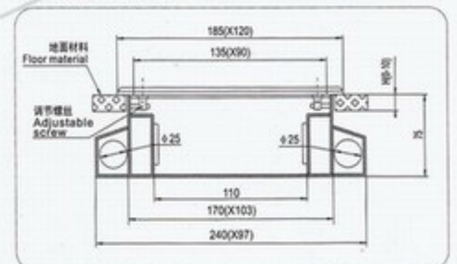
外形及安装尺寸 / Overall and installation size
