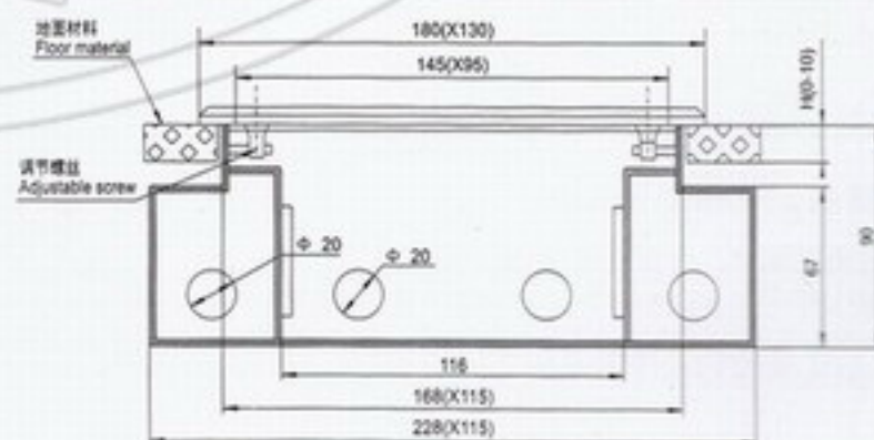
外形及安装尺寸 / Overall and installation size
